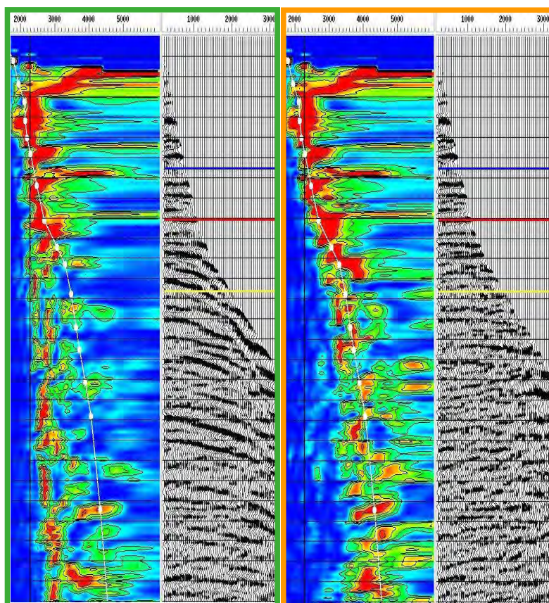
Velocity analysis on the land seismic data before multiple attenuation
